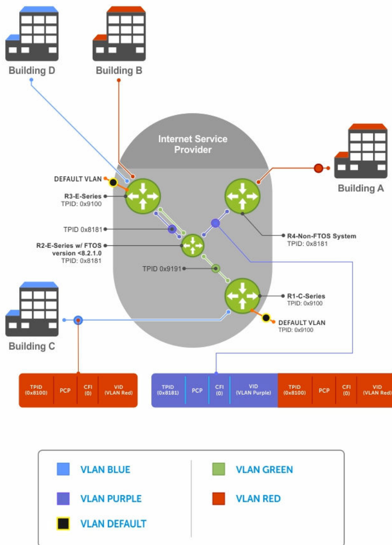
Figure 107. Single and Double-Tag TPID Mismatch
